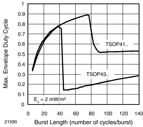
21590 Burst Length (number of cycles/burst) Fig. 9 - Max. Envelope Duty Cycle vs. Burst Length
